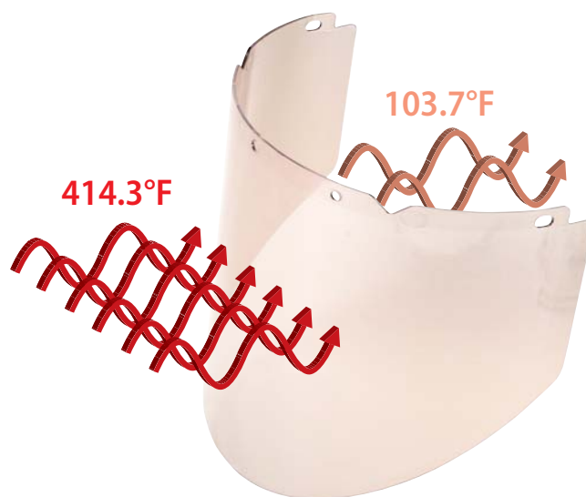
Figure 1: V-Gard Reflective-Coated Visor surfaces were exposed to irradiance of 9.5kW/m 2 . For comparative purposes, firefighters are typically exposed to radiant heat fluxes between 5-10 kW/m 2 during a fire. 4
